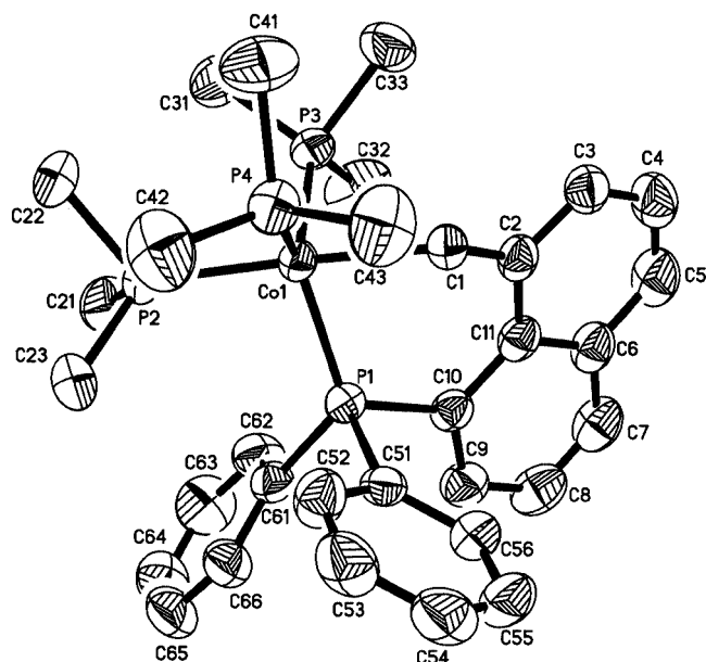
Figure 2. Molecular structure of 4 (ORTEP plot with hydrogen atoms omitted); selected bond lengths [Å] and angles [°]: Co–C1 2.090 (3), Co–P1 2.1438(9), Co–P2 2.1904(12), Co–P3 2.1932(10), Co–P4 2.2180(11), P1–C10 1.859(3), C10–C11 1.421(4), C2–C11 1.420(4), C1–C2 1.484(4); C1–Co–P1 79.72(9), C1–Co–P2 176.61(10), C1–Co–P3 88.32(10), C1–Co–P4 85.25(9), P1–Co–P2 98.60(4), P1–Co–P3 120.87(4), P1–Co–P4 121.21(4), P2–Co–P3 95.06(4), P2–Co–P4 93.18(4), P3–Co–P4 115.02(4), Co–P1–C10 117.05(10), P1–C10–C11 120.4(2), C2–C11–C10 123.5(2), C11–C2–C1 121.7(3), Co–C1–C2 123.4(2).
